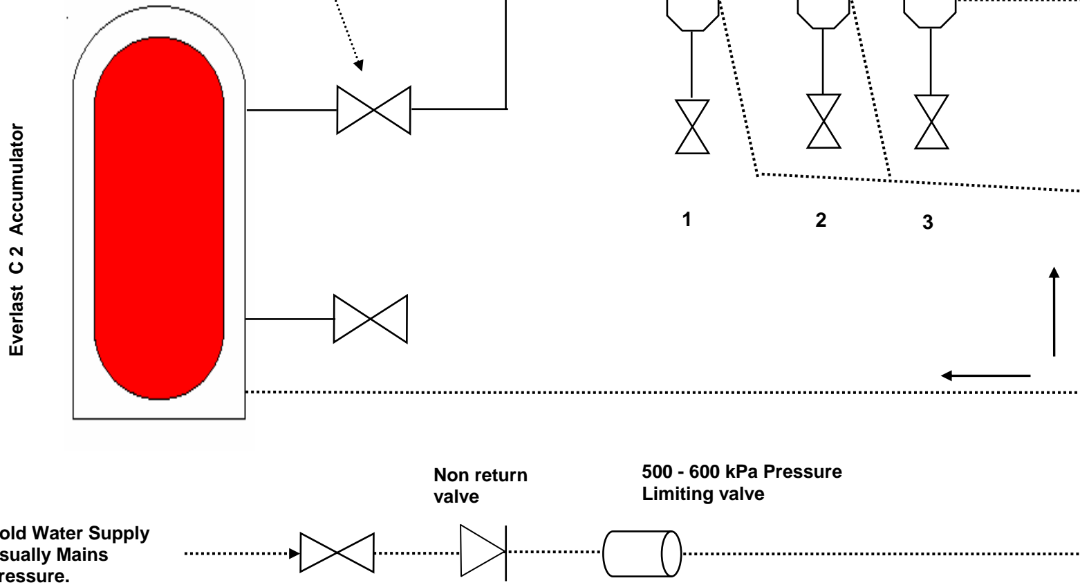
DIAGRAM 1. WATER MAINS PRESSURE CIRCUIT
