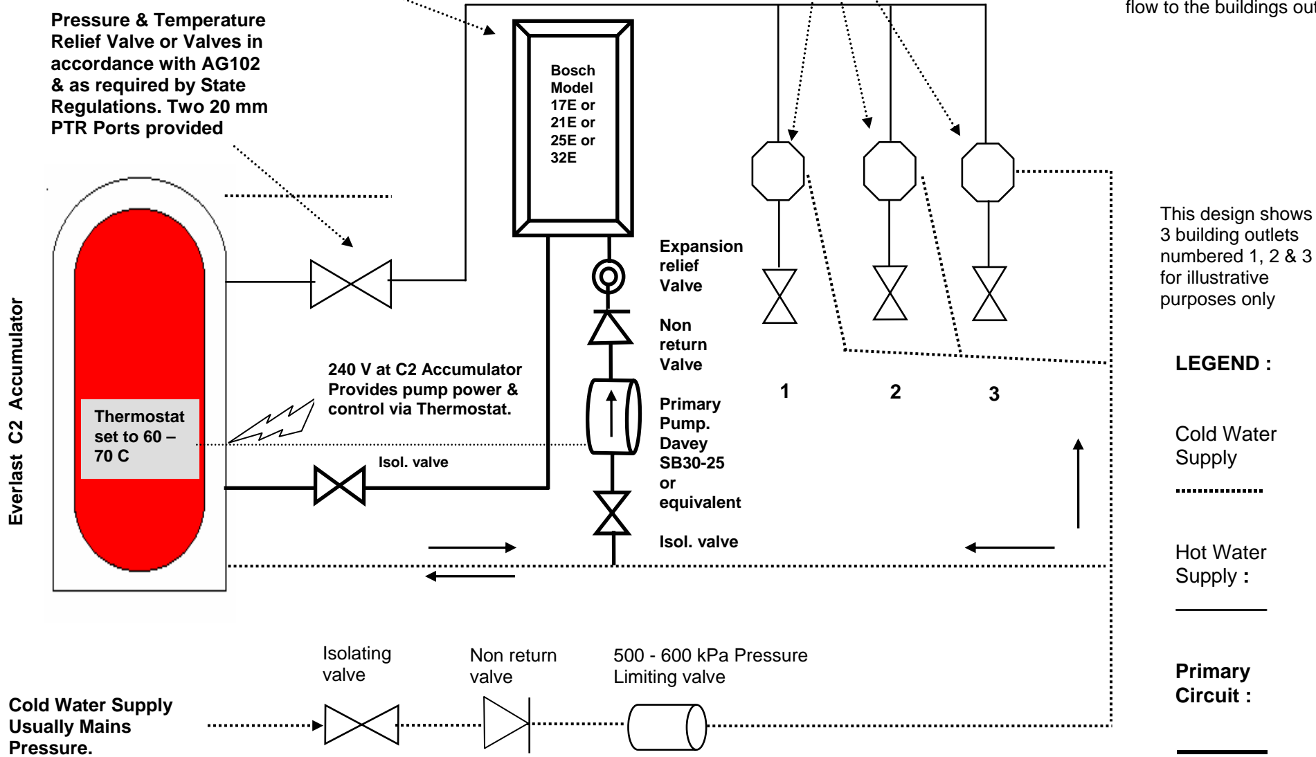
DIAGRAM 2. WATER MAINS PRESSURE plus PRIMARY CIRCUIT
